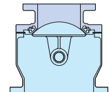
DVET Dome Valve® TOP INLET ADAPTOR Inlet and outlet sides pressure tight up to 7 bar(g)
