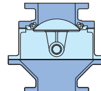
DVI Dome Valve® IN-LINE Inlet and outlet sides pressure tight up to 7 bar(g)
