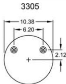
BEAD PLATE TOP
